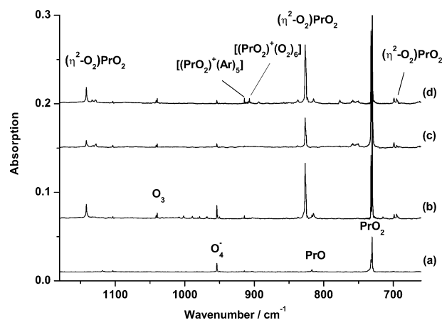
Figure 3. Infrared absorption spectra in the 1180\text{--}660\text{ cm}^{-1} region of praseodymium oxide species obtained from co-deposition of laser-evaporated Pr atoms with 0.1% \text{O}_2 in argon. a) 1 h of sample deposition at 4 K, b) after 25 K annealing, c) after 15 min of UV light irradiation, and d) after 30 K annealing.
